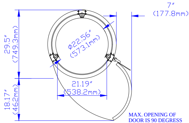
VIEW "A-A"
