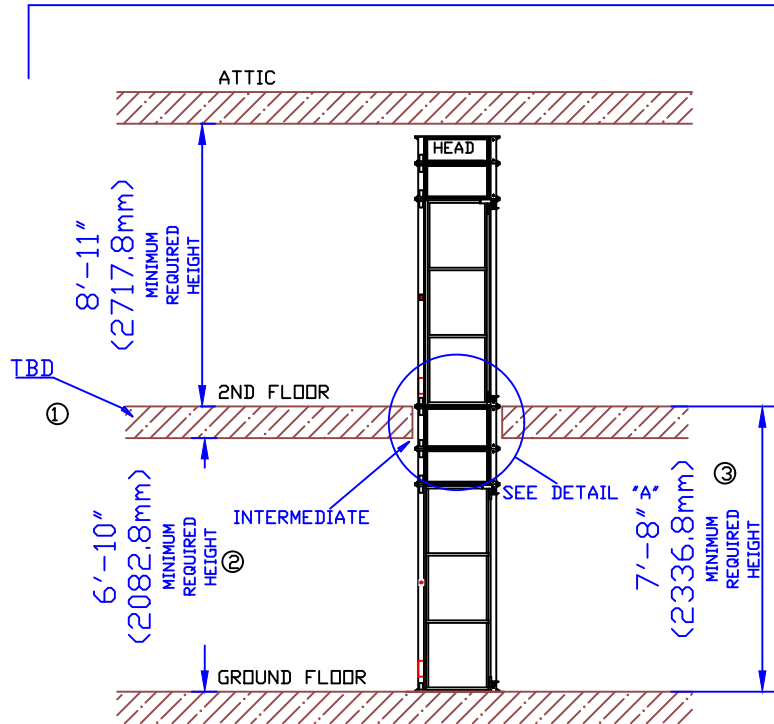
VIEW "A-A"
